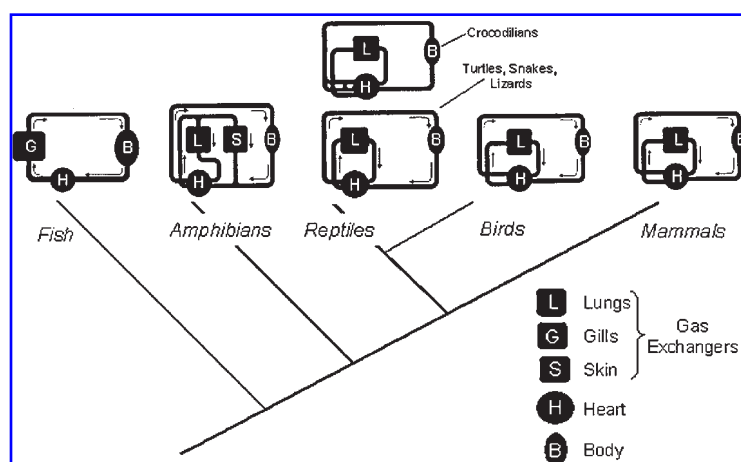
FIG. 2. General schematics of the vertebrate circulatory patterns, showing the relations between the heart and the gas-exchange organs(s) of each circulation. From Burggren and Reiber (2006) after Hicks (2002).
