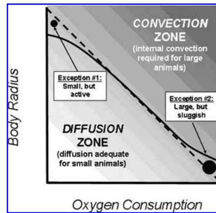
FIG. 1. The relation between body size, metabolic rate, and the ability of simple diffusion to provide adequate oxygenation of small animals. Generally, animals falling in the “diffusion zone” on this figure can supply all of their oxygen needs by diffusion, but as body size or metabolic rate or both increase, the need for an internal convection of body fluids increases. Exceptions are large animals with unusually low metabolic rates, or small animal with unusually large metabolic rates. (From Burggren and Reiber, 2007).
