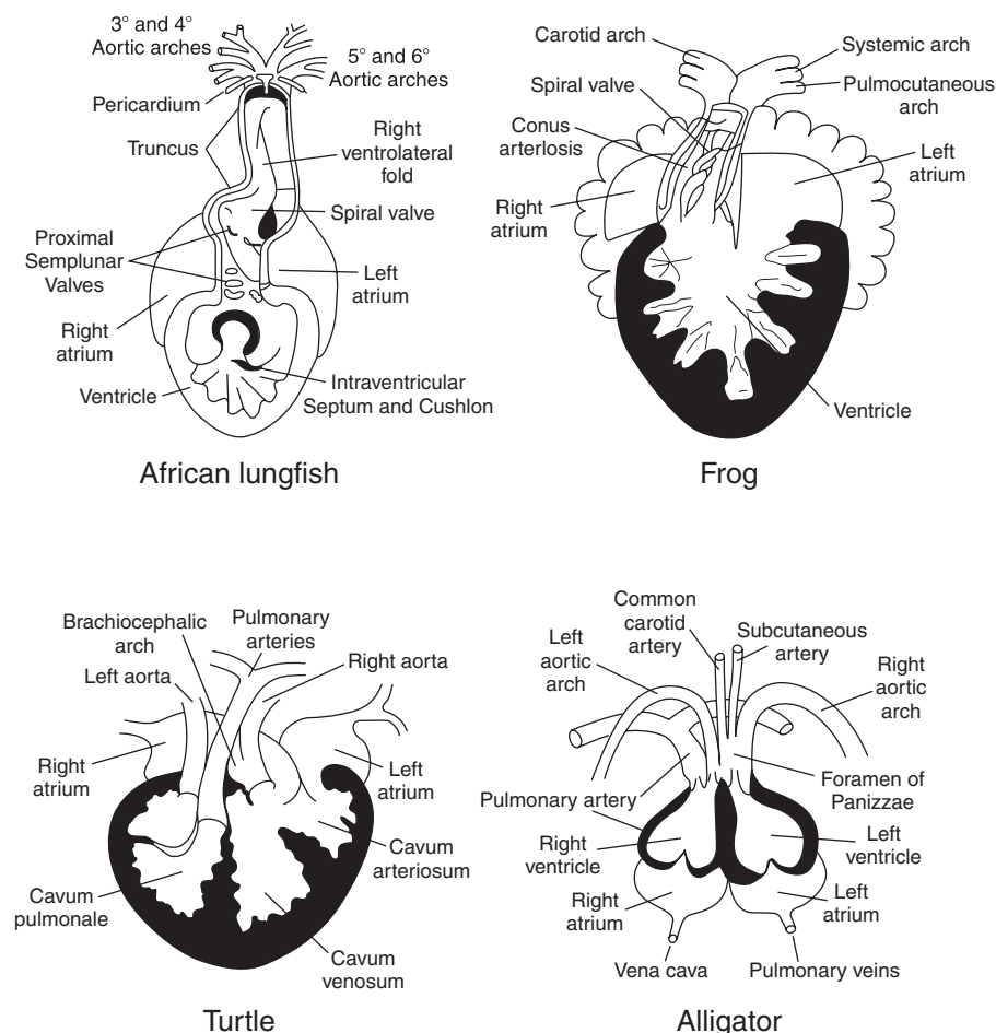
FIG. 3. Gross morphology of the outflow tract(s) of the heart of representative lower vertebrates. The patterns of flow of oxygenated and deoxygenated blood through each of these hearts is surprisingly complex, involving both spatial and temporal components to maintaining separation of bloodstreams. (For description of blood-flow patterns and literature sources, see Burggren et al. , 1997).
