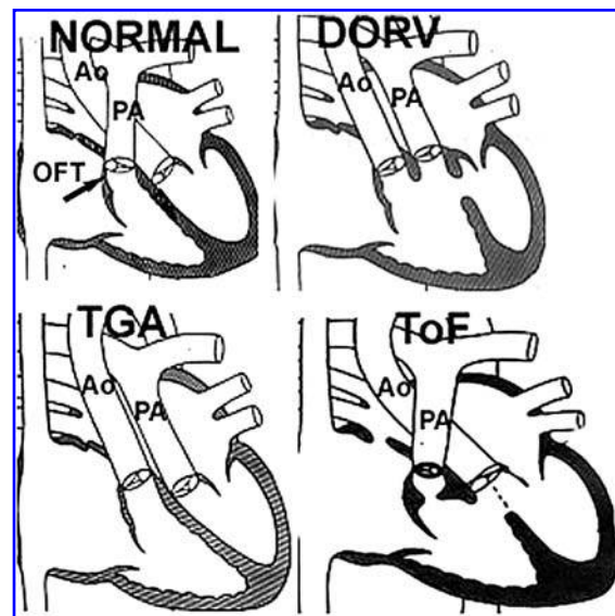
FIG. 4. Congenital defects in the human cardiac outlet structures (conotruncus) that result in right-to-left shunting of deoxygenated blood. These defects are postulated to arise from malrotation of the OFT or myocardial infundibular defects or both. DORV, Double-outlet right ventricle. Both great vessels (Ao, aorta; and PA, pulmonary artery) connect via the myocardial infundibulum to the right ventricle. TGA, Transposition of the great arteries. The Ao connects via the infundibulum to the RV, and the PA directly connects to the LV. ToF, Tetralogy of Fallot. Pulmonic stenosis is secondary to infundibular hypoplasia, and the aorta is malrotated and thus partially overrides the right ventricle. These defects are associated with ventricular septal defects, which provide a necessary conduit for blood flow. Although shown as individual entities, these dysmorphologies represent a spectrum of defects in the conotruncal structures.
