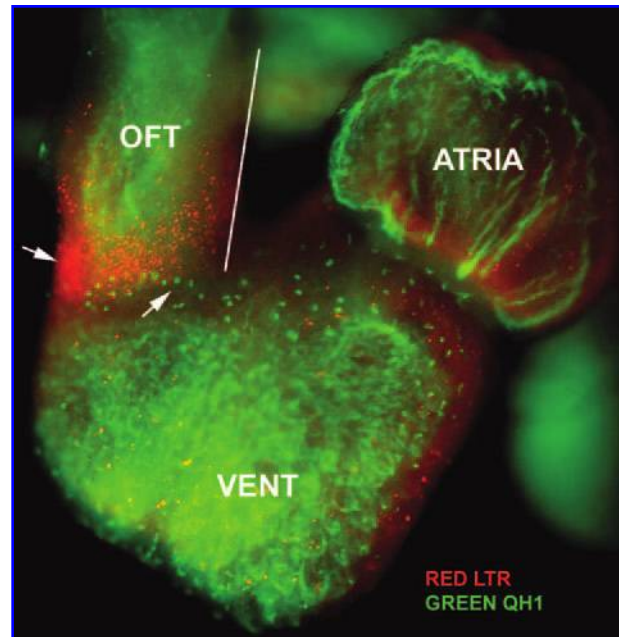
FIG. 6. Key cellular processes in avian heart morphogenesis. OFT cardiomyocytes are eliminated by apoptosis, as indicated by LysoTracker Red (LTR) staining (arrow), observed in this whole-mount picture of a stage 25 quail heart. Endothelial progenitor cells, detected with an anti-QH1 antibody, are observed within the epicardial tissue covering the ventricle (arrow) and are recruited to the OFT, where they will be organized into a vascular network. The chamber endocardial endothelium is also QH1 positive. (For interpretation of the references to color in this figure legend, the reader is referred to the web version of this article at www.liebertonline.com/ars )
