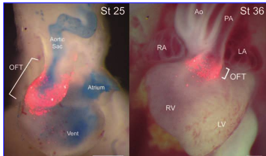
FIG. 5. Avian heart development: transition from the more-primitive single circulation (stage 25, ED5) to the mature dual in-series configuration (stage 36, ED10). Development and remodeling of the embryonic chick cardiac OFT (A). The OFT myocardium of the stage 25 (ED5) and stage 36 (ED10) chick heart is labeled with red fluorescent protein expressed from recombinant adenovirus. The lumens of the hearts and vessels are filled with blue ink in (A) and blood in (B). In this developmental window (1), the OFT myocardium shortens and commits to the right heart, forming the subpulmonic infundibulum. The OFT rotates, placing the aorta in a posterior position to connect with the
